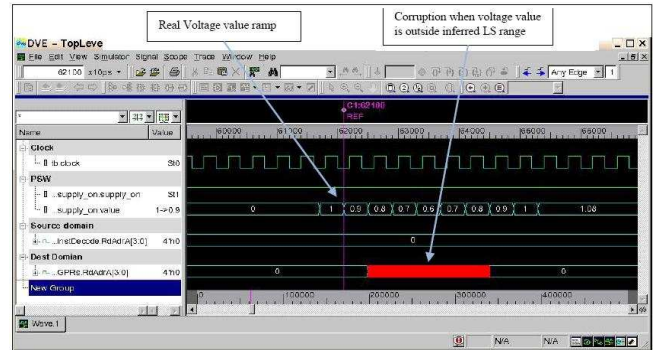
Figure 9. Level Shifter Corruption when Voltage Change
