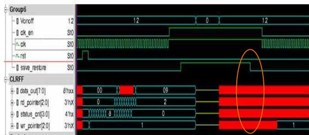
Figure 8. Failed Control Sequence for Custom Retention
