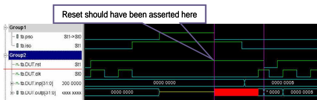
Figure 7 Power On Reset Assertion Sequence
